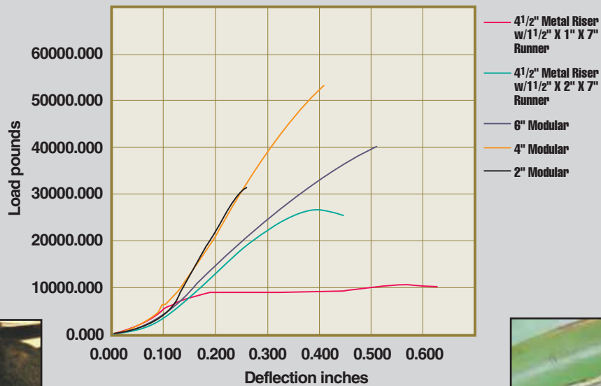
Runner Load X Deflection Test
